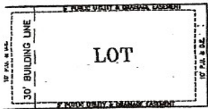
TYPICAL LOT DETAIL
